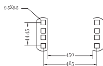
19" mounting
